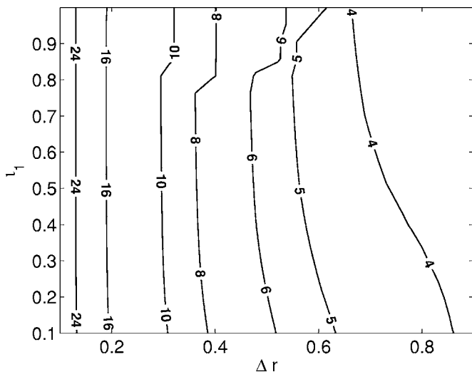
FIG. 3. Contour plot of spacing between lowest eigenvalues \Delta\lambda_2 as a function of interface separation \Delta r = r_2 - r_1 and \epsilon_1 . The contour labels display the value of \Delta\lambda .
