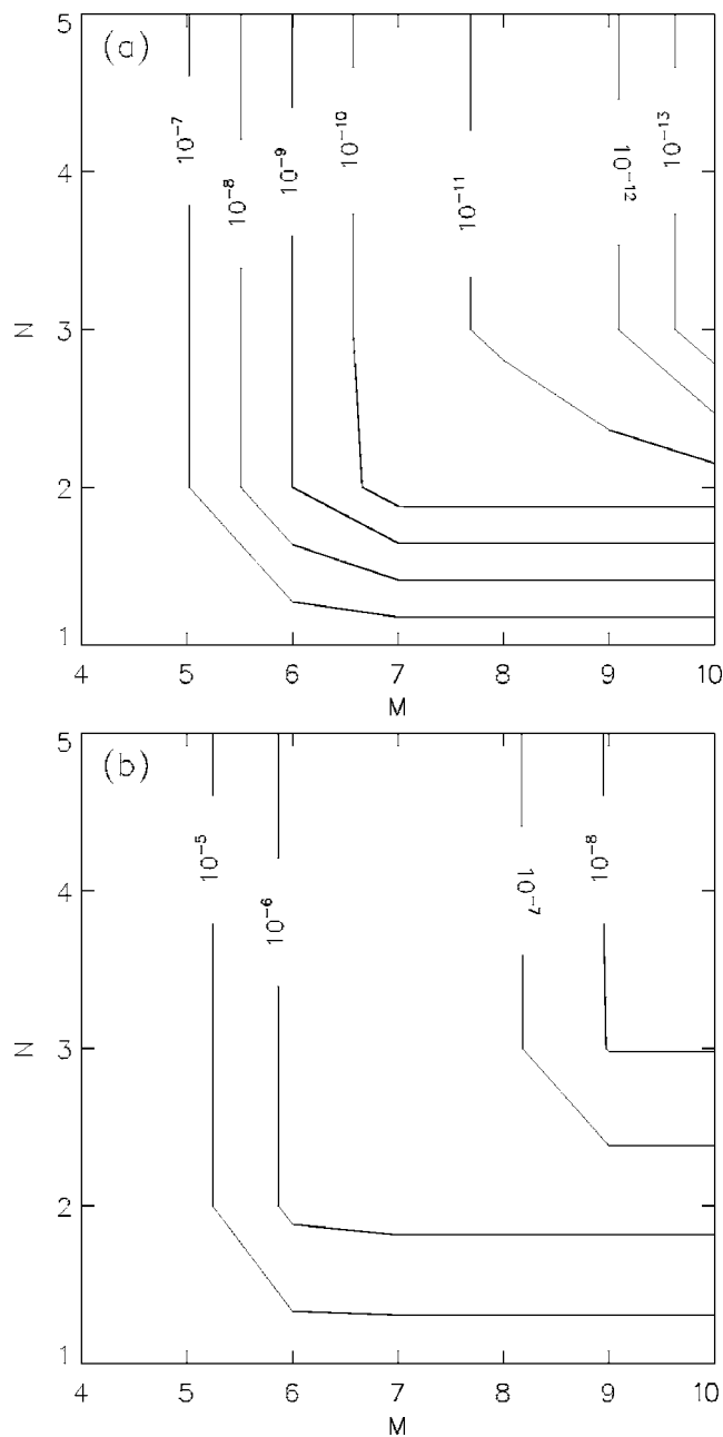
FIG. 4. Fourier convergence error: (a) |\delta s| , and (b) |\delta \dot{\theta}| , for the configuration with \delta=0.0015 .
